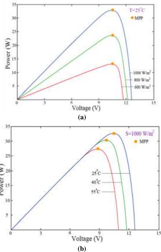
Fig. 1. The output power-voltage curve; a) constant temperature and variable radiation; b) constant radiation and variable temperature
